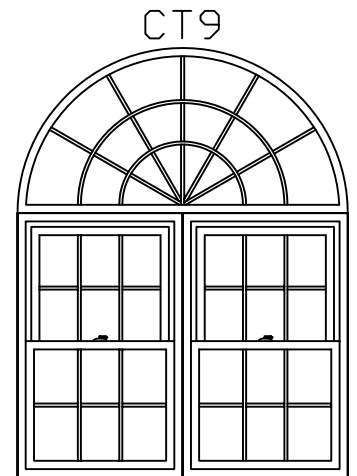
CT9 LARGE TWIN DOUBLE HUNG SHOWN WITH HALF ROUND WITH CT9 DOUBLE SUNBURST. RECOMMENDED OVER TWIN DOUBLE HUNGS RANGING IN WIDTH FROM 47 1/4' TO 60'. HALF ROUND SHOWN WIDTH = 60' HEIGHT = 30'
