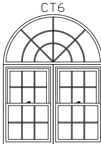
CT6 LARGE TWIN DOUBLE HUNG SHOWN WITH HALF ROUND WITH CT6 DOUBLE SUNBURST. RECOMMENDED OVER TWIN DOUBLE HUNGS RANGING IN WIDTH FROM 47 1/4' TO 60'. HALF ROUND SHOWN WIDTH = 60' HEIGHT = 30'
