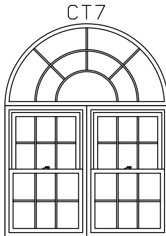
CT7 LARGE TWIN DOUBLE HUNG SHOWN WITH HALF ROUND WITH CT7 DOUBLE SUNBURST. RECOMMENDED OVER TWIN DOUBLE HUNGS RANGING IN WIDTH FROM 47 1/4' TO 60'. HALF ROUND SHOWN WIDTH = 60' HEIGHT = 30'
