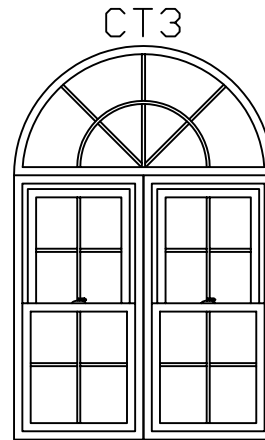
CT3 SMALL TWIN DOUBLE HUNG SHOWN WITH HALF ROUND WITH CT3 SUNBURST. RECOMMENDED OVER TWIN DOUBLE HUNGS RANGING IN WIDTH FROM 36' TO 47'. HALF ROUND SHOWN WIDTH = 47' HEIGHT = 23 1/2'
